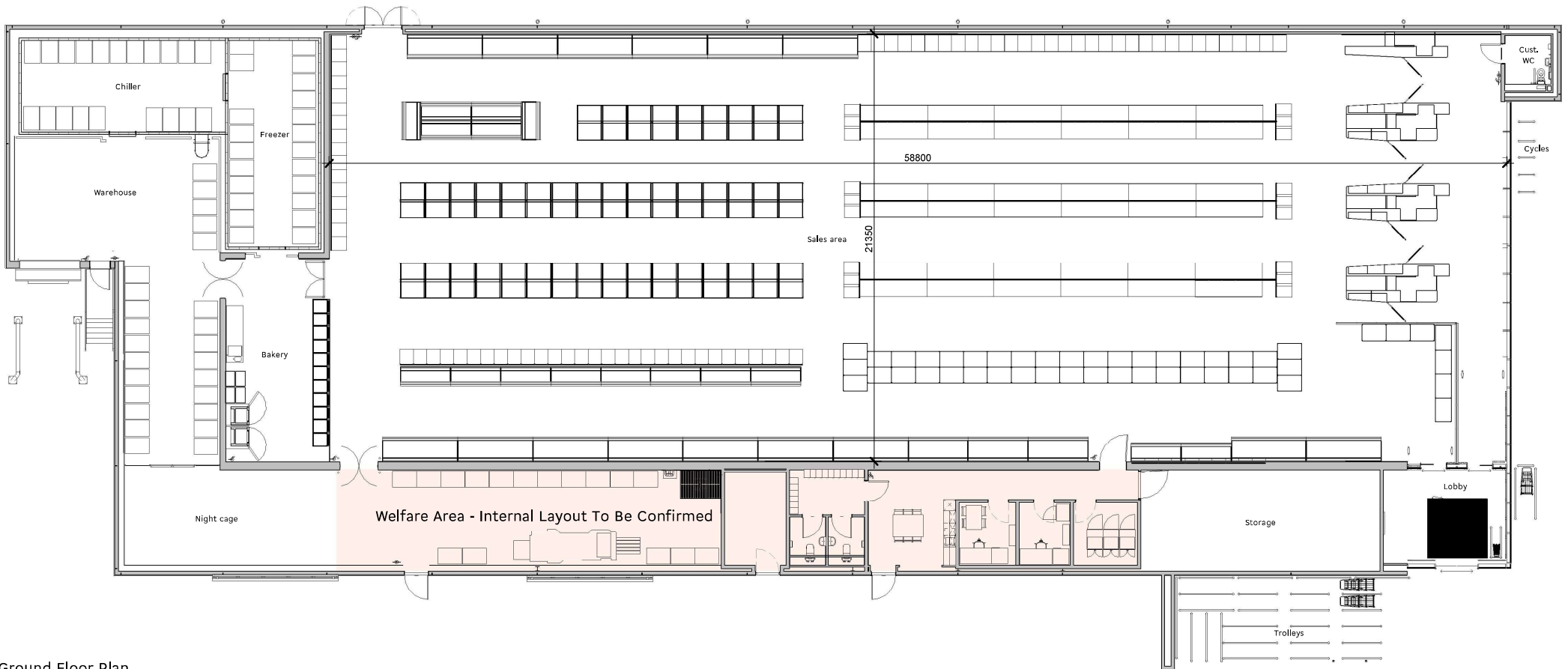
Ground Floor Plan 1 : 200
